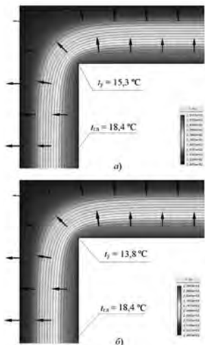
Figure 1. Temperature fields in an outer corner of a single-layer outer wall a) for \alpha_i = 8.7 W/(m 2 •K), b) for \alpha_i = 5.8 W/(m 2 •K)
