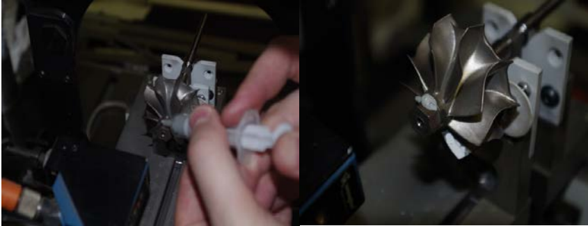
Fig. 12. Imposition of mass on the turbine wheel 13. Imposition of mass on the turbine wheel
