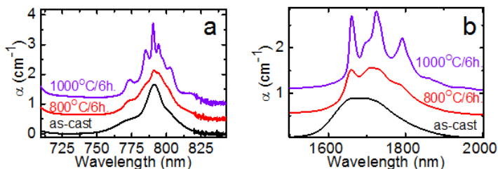
Fig. 1 - Absorption of \text{Tm}^{3+} ions related to the transitions to {}^3\text{H}_4 (a) and {}^3\text{F}_4 (b) states for initial glass and GCs heat-treated at 800^\circ\text{C} and 1000^\circ\text{C} .
