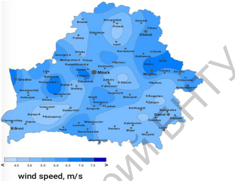
Figure 2 – Average design wind speed at a height of 100 m
